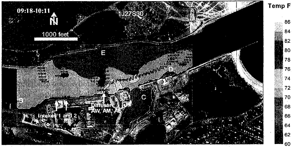
Figure 3.17 Contours of surface temperatures between 09:18 – 10:11 on 27 July 1999.
