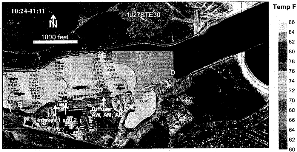
Figure 3.18 Contours of surface temperatures between 10:24 – 11:11 on 27 July 1999.
